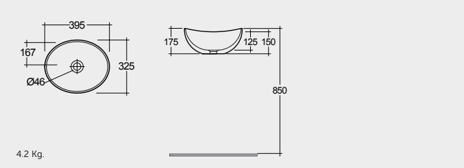
39 CM OC161AWHA Bowl | حوض
