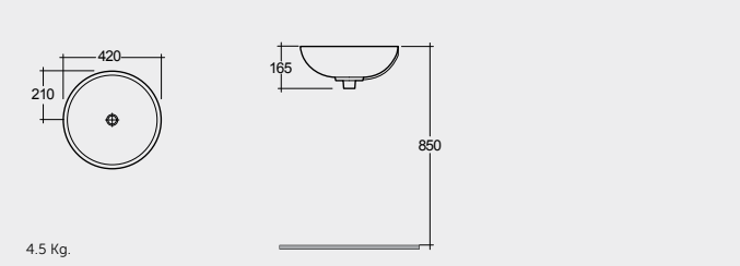
42 CM OC72AWHA Bowl | حوض
