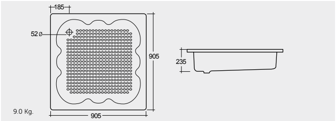
90x90 CM SH05AWHA
