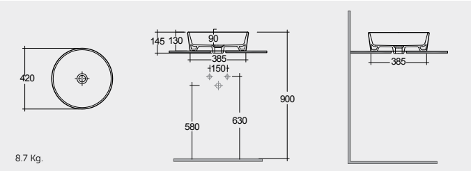
42 CM HAR106AWHA Round | دائري
