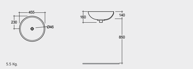
45 CM OC137AWHA Bowl | حوض
