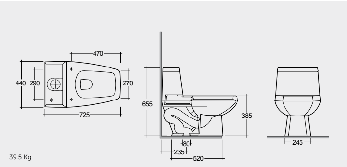
SIPHONIC ONE PIECE WC 73 CM
