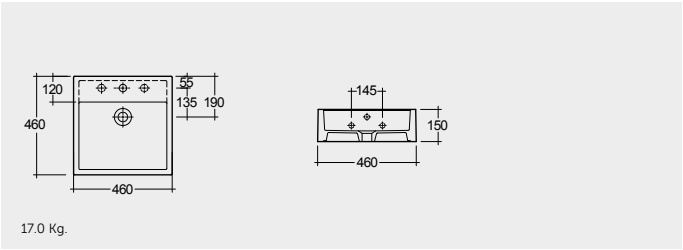
CLOAKROOM WASH BASIN 46 CM
