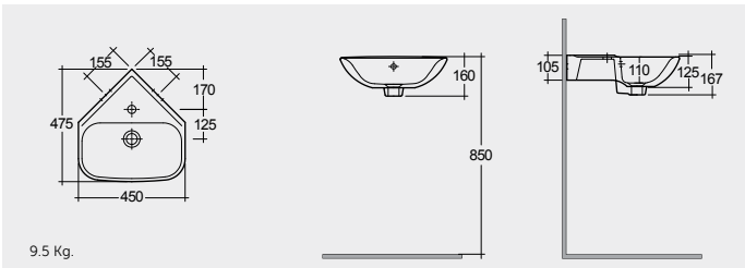
CORNER CLOAKROOM WASH BASIN 45 CM
