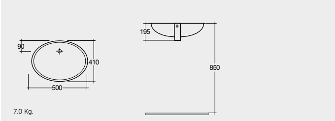
UNDER COUNTER WASH BASIN 50 CM
