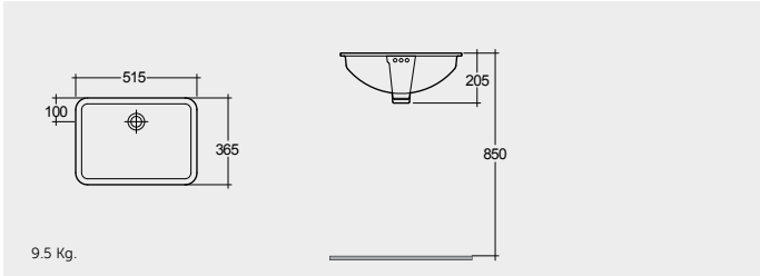
UNDER COUNTER WASH BASIN 51 CM
