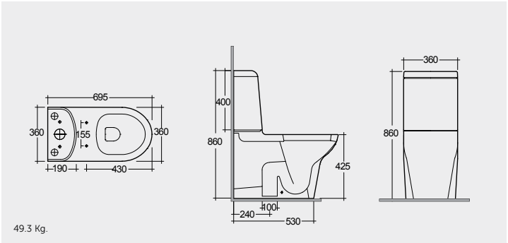
CLOSE COUPLED WC (S) TRAP 69 CM
