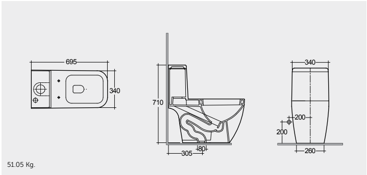
DELUXE SIPHONIC ONE PIECE WC 69 CM
