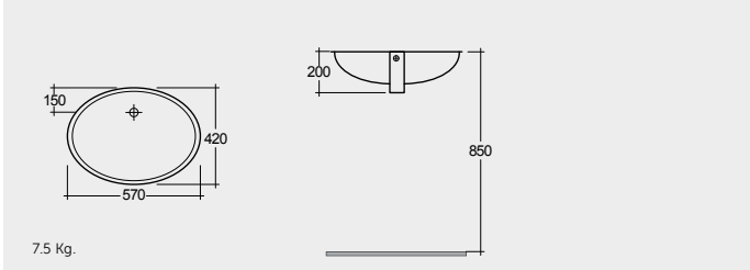
UNDER COUNTER WASH BASIN 57 CM
