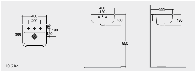
CLOAKROOM WASH BASIN 40 CM
