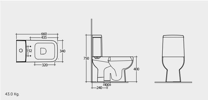
RIMLESS ONE PIECE WC 66 CM
