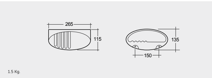
BIG SOAP HOLDER
