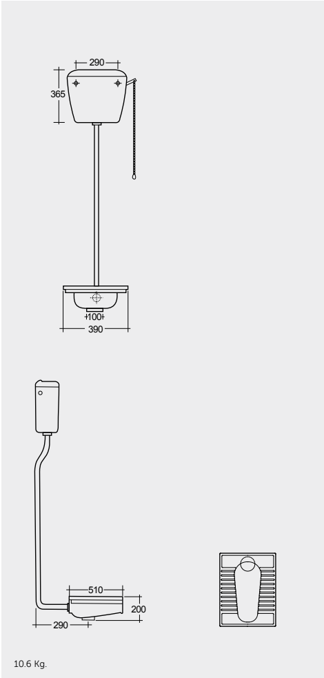
SQUATTING PAN AND CISTERN DELUXE
