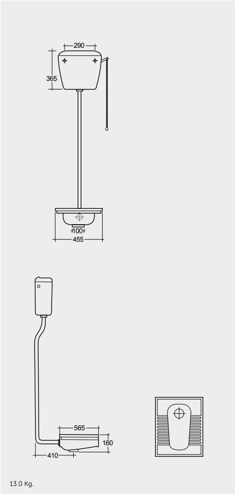
SQUATTING PAN AND CISTERN 13 CM
