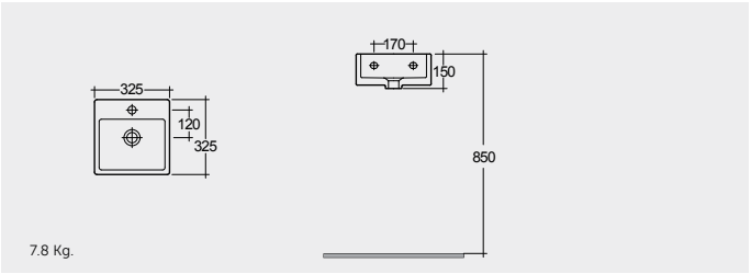
CLOAKROOM WASH BASIN 32 CM
