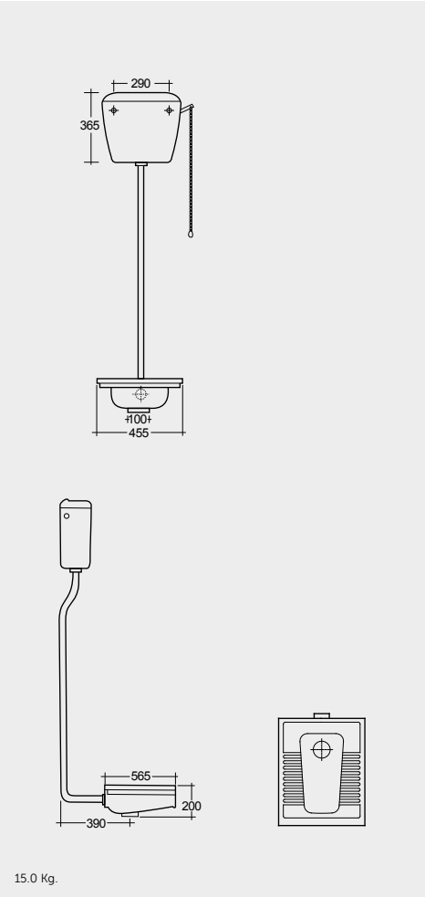
SQUATTING PAN AND CISTERN 18 CM
