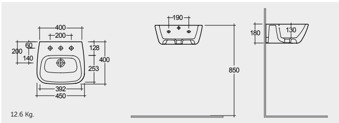
CLOAKROOM WASH BASIN 45 CM
