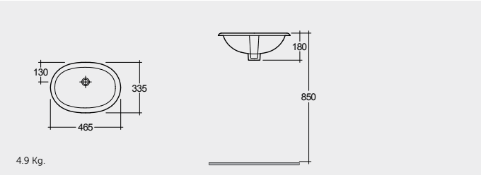
UNDER COUNTER WASH BASIN 46 CM
