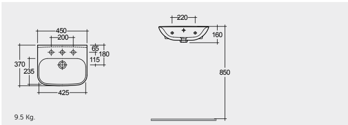
CLOAKROOM WASH BASIN 45 CM
