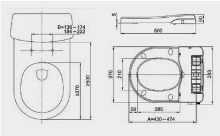
CLOSE COUPLED WC (P) TRAP (BACK OPEN) 65 CM WITH BIDET FUNCTION SEAT COVER
