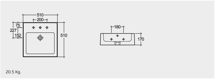
CLOAKROOM WASH BASIN 51 CM
